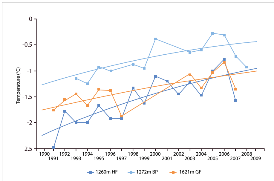
Figure 2. Permafrost temperature from the three most continuous stations in the Mackenzie Mountain research area, Canada. The trend clearly indicates warming over the record period. HF=Hare Foot; BP=Beaver Pond; GF=Goose Flats; m=height above sea level in meters.
