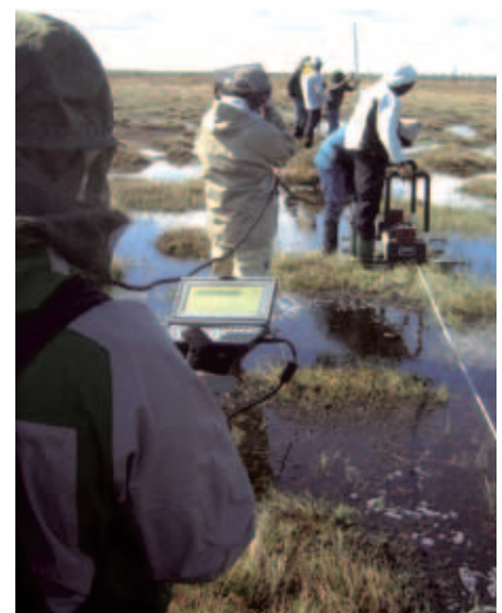
Volunteers conduct ground-penetrating radar surveys along transects to measure permafrost thickness.
